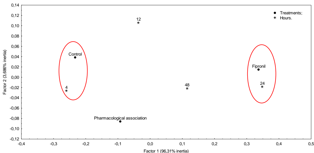
Figure 2 - Behavior patterns between the treatments and the periods analyzed for control of P. spinulosa in wistar rats by correspondence analysis.
