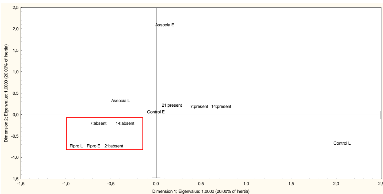
Figure 3 - Patterns between treatments: pharmacological association (Associa), Fipronil (Fipro) and control (Control) for presence or absence of lice (L) and eggs (E) over the days analyzed: 7, 14 and 21 days in wistar rats naturally parasitized by P. spinulosa in correspondence analysis.
